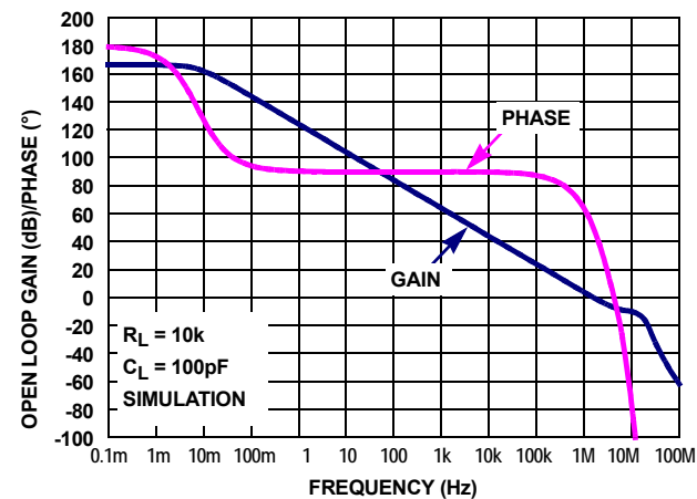
FIGURE 39. OPEN-LOOP GAIN, PHASE vs FREQUENCY, R_L = 10k\Omega, C_L = 100pF
