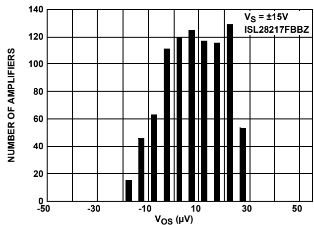
FIGURE 4. V_{OS} DISTRIBUTION FOR GRADE B
